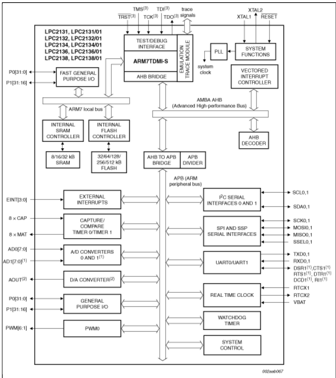
Block diagram: LPC2131FBD64, LPC2132FBD64, LPC2132FHN64, LPC2134FBD64, LPC2136FBD64, LPC2138FBD64, LPC2138FHN64 Block Diagram
