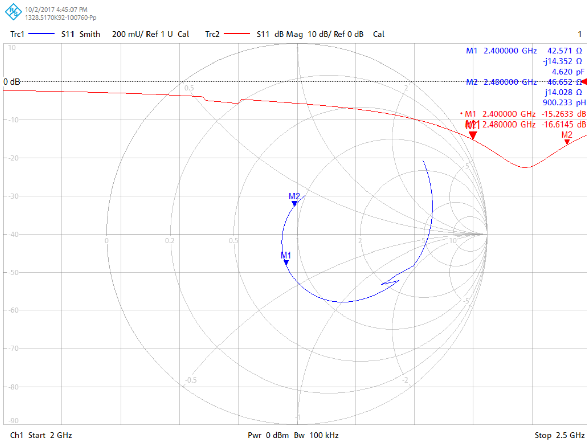
Figure 58. S11 diagram (Tx mode)
