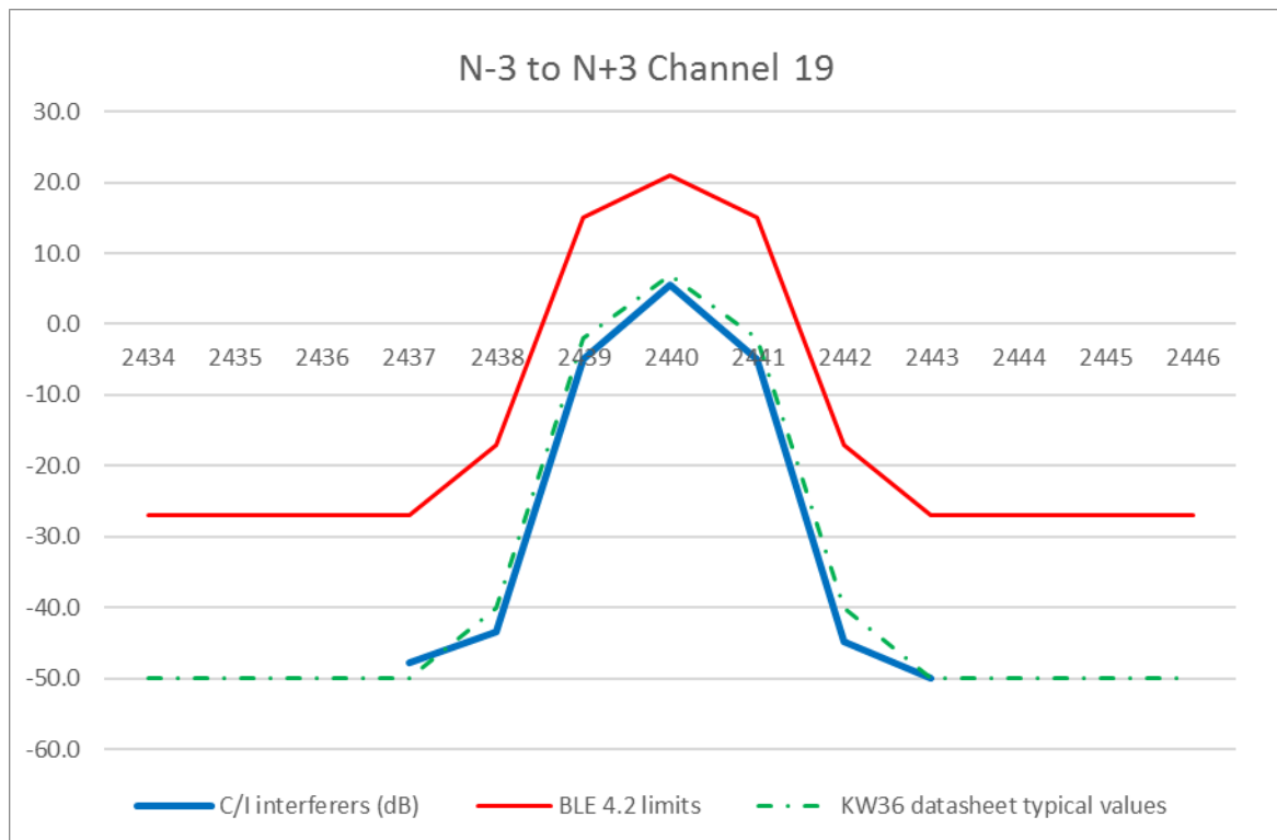
Figure 53. Adjacent, alternate, and co-channel rejection (channel 19)
