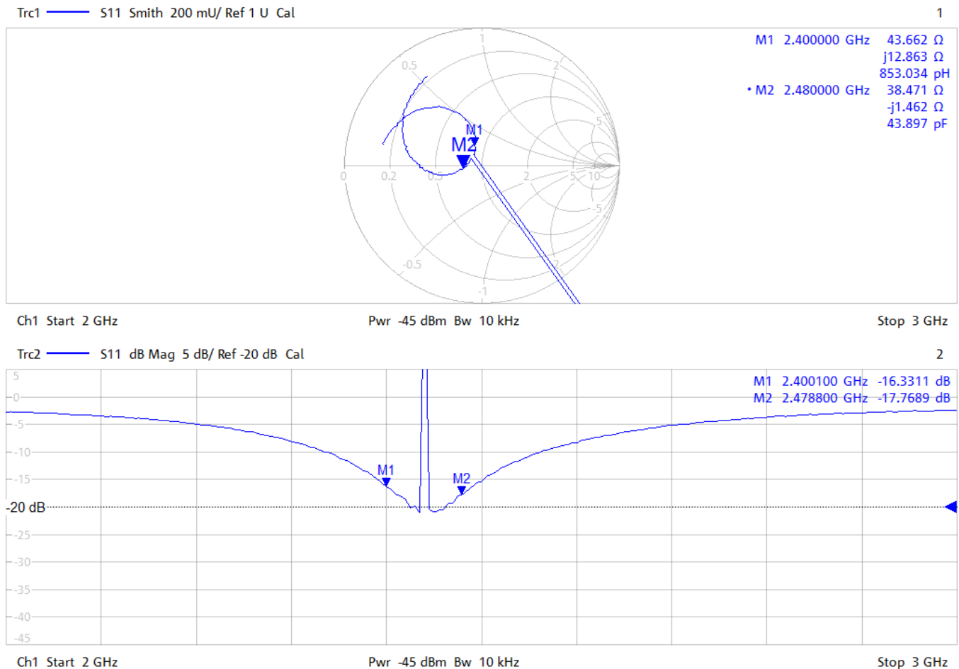
Figure 60. S11 diagram (Tx mode)
