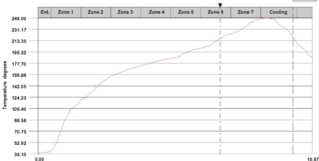
Figure 15. Typical Solder Reflow Profile for Pb-free SnAgCu Solder
