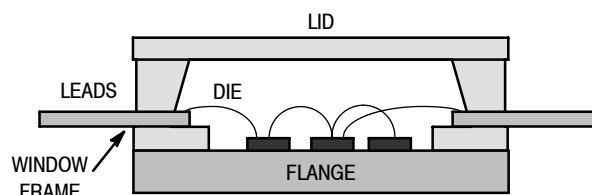
Figure 3. Air Cavity Package Construction for Power Devices
