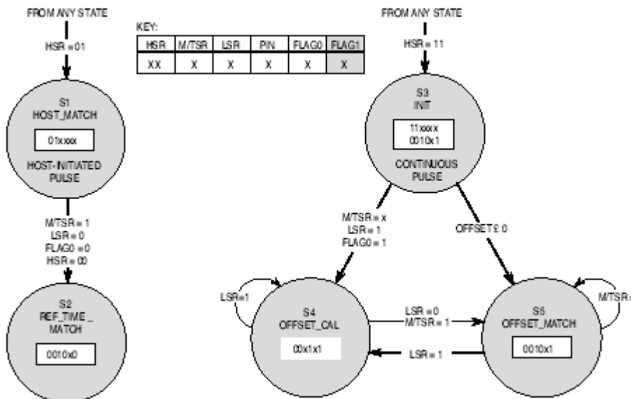
Figure 5. Output Compare State Flowchart
