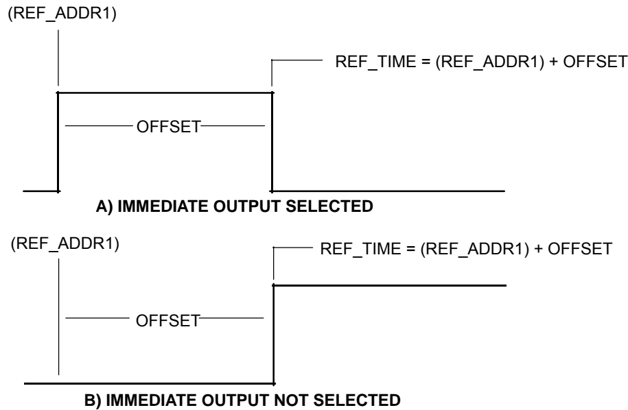
Figure 1. Host-Initiated Pulse Mode Diagram
