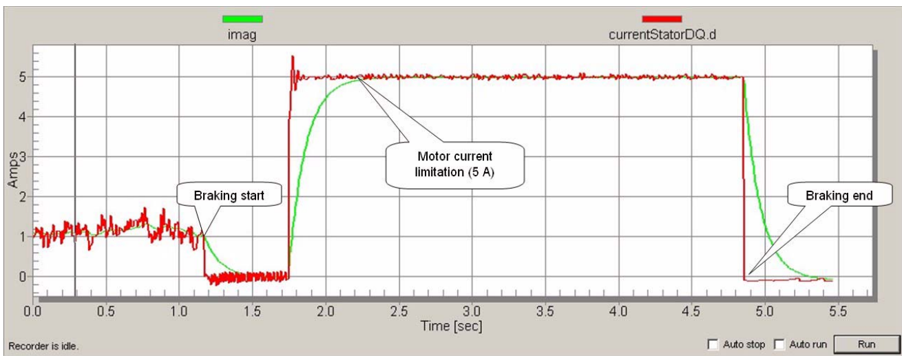
Figure 20. Non-Recuperative Braking
