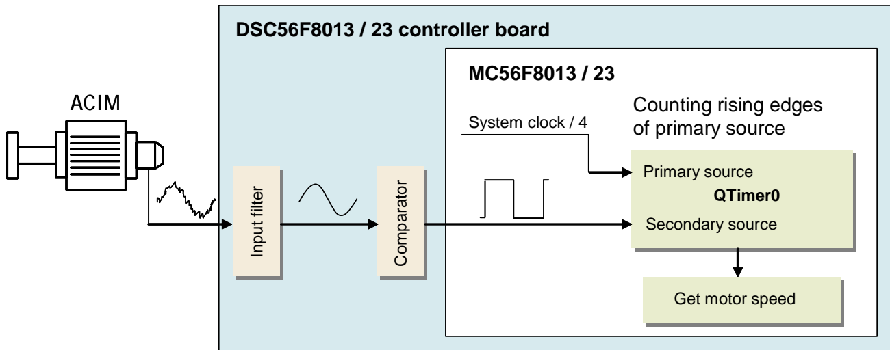
Figure 12. Speed Sensing Using Hardware Comparator Concept
