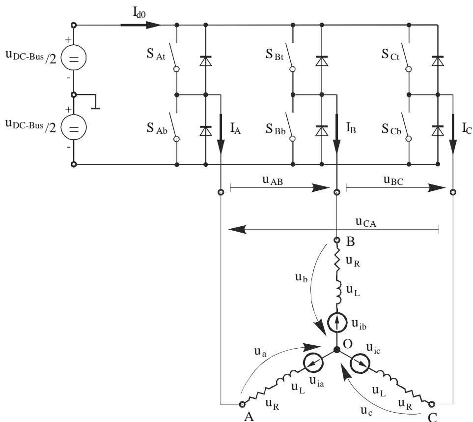
Figure 6. Three-Phase Voltage Source Inverter
