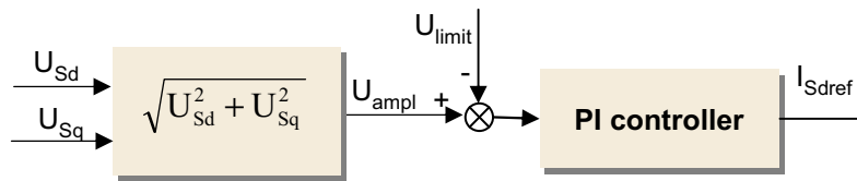
Figure 11. Internal Structure of Field-Weakening Block
