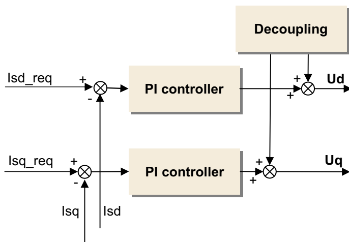
Figure 9. Current Controller Loop
