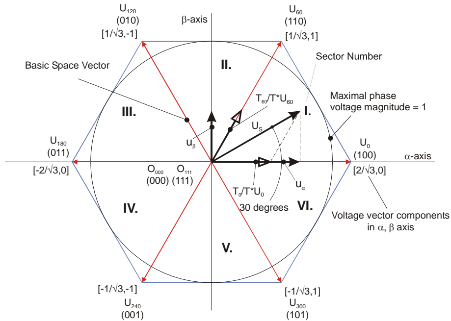
Figure 7. Basic Space Vectors and Voltage Vector Projection
