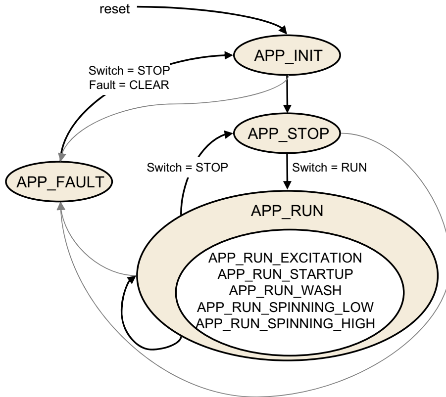
Figure 17. Application State Diagram
