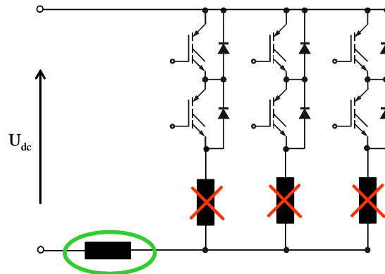
Figure 10. Single Shunt Sensing Approach
