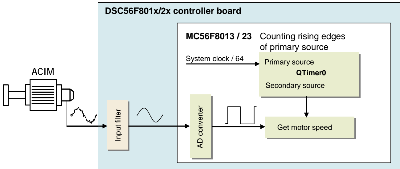
Figure 13. Speed Sensing Using Software Comparator Concept
