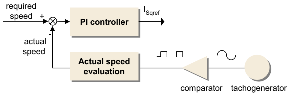
Figure 14. Speed Control Loop
