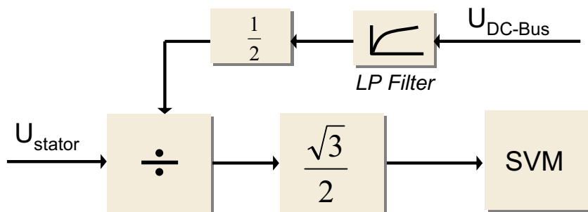
Figure 8. DC-Bus Ripple Elimination
