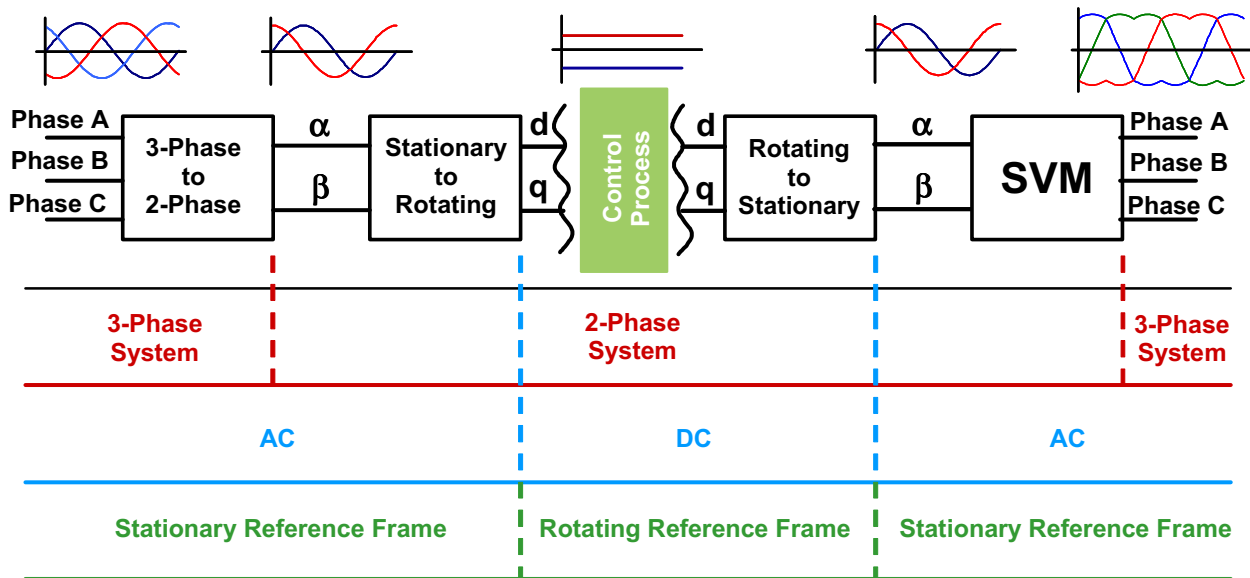
Figure 2. Vector Control Transformations
