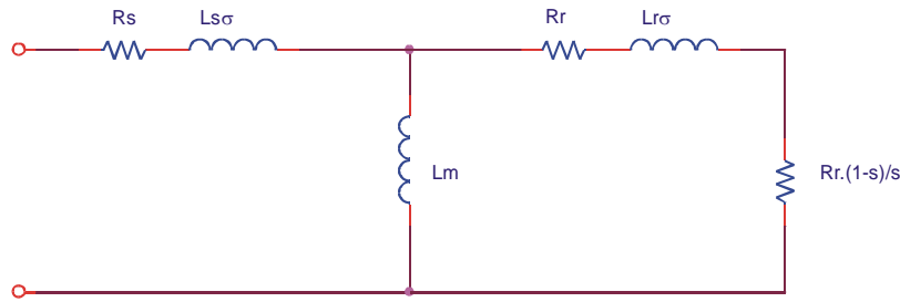
Figure 3. Induction Motor Equivalent Circuit
