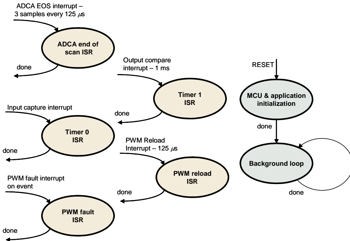
Figure 16. Software Flowchart
