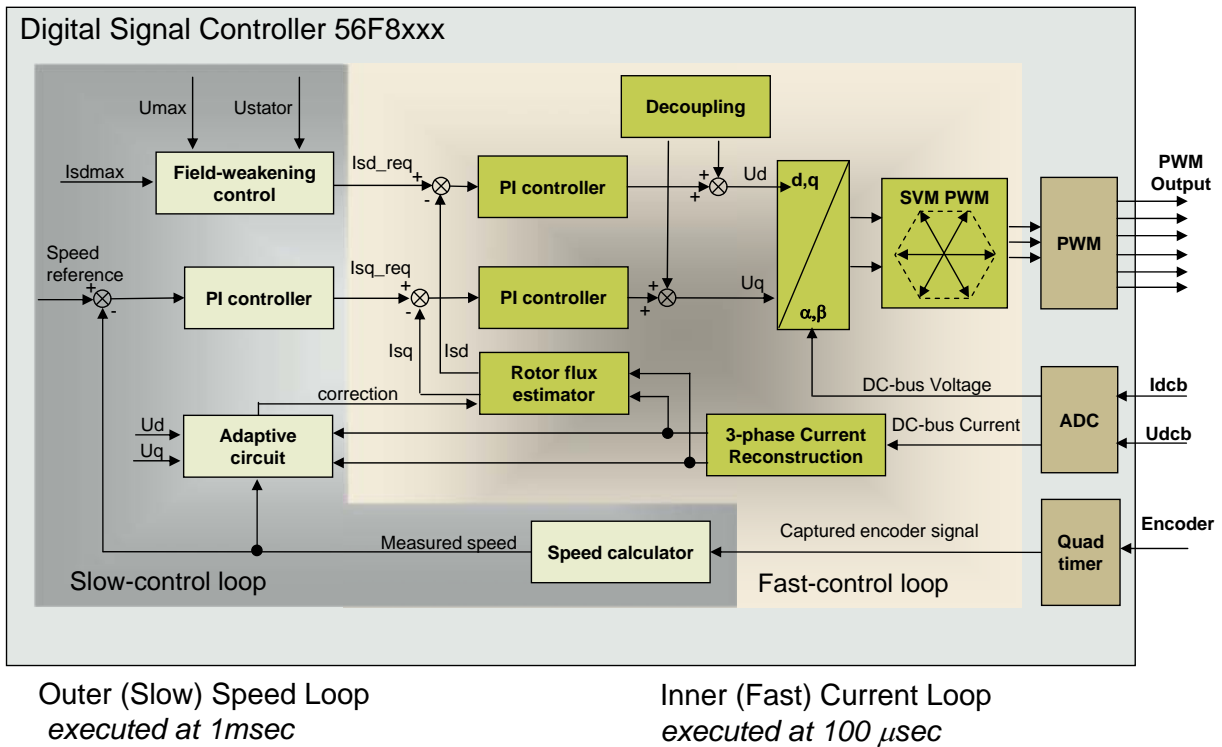
Figure 5. Control Algorithm Overview
