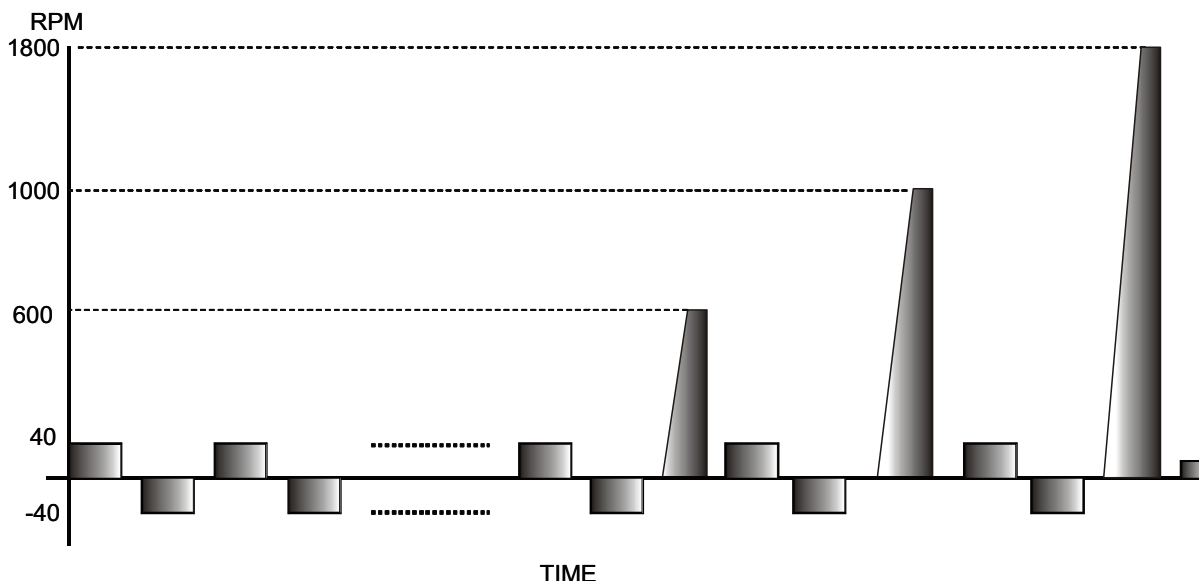
Figure 15. Speed Profile of the Washing Cycle
