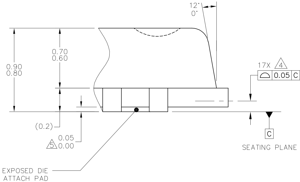
DETAIL G VIEW ROTATED 90° CW
