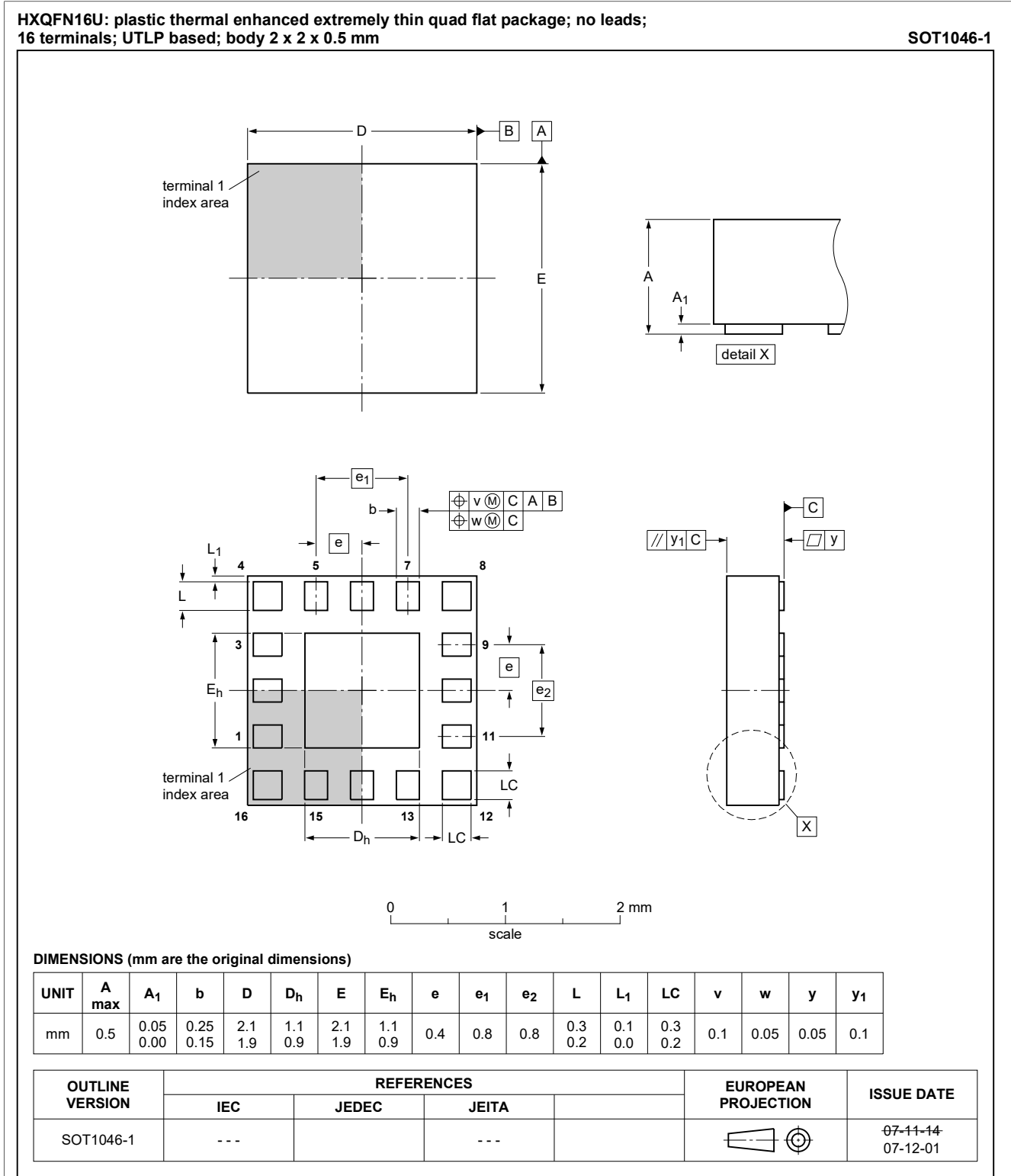
Figure 1. Package outline HXQFN16U (SOT1046-1)
