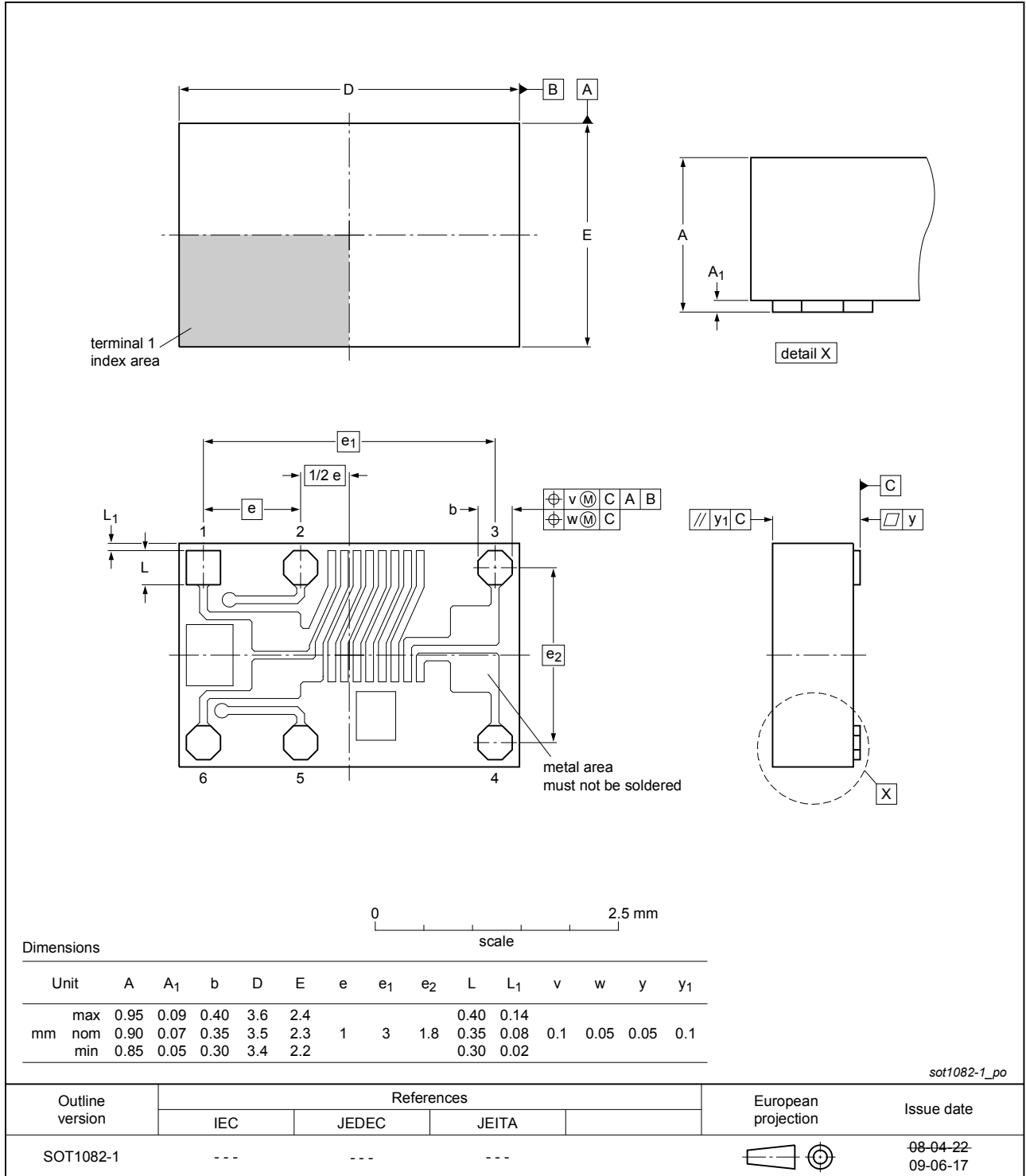
Fig. 1. Package outline VSON6U (SOT1082-1)
