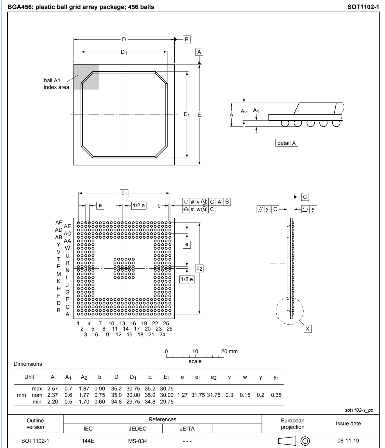
Fig. 1. Package outline BGA456 (SOT1102-1)
