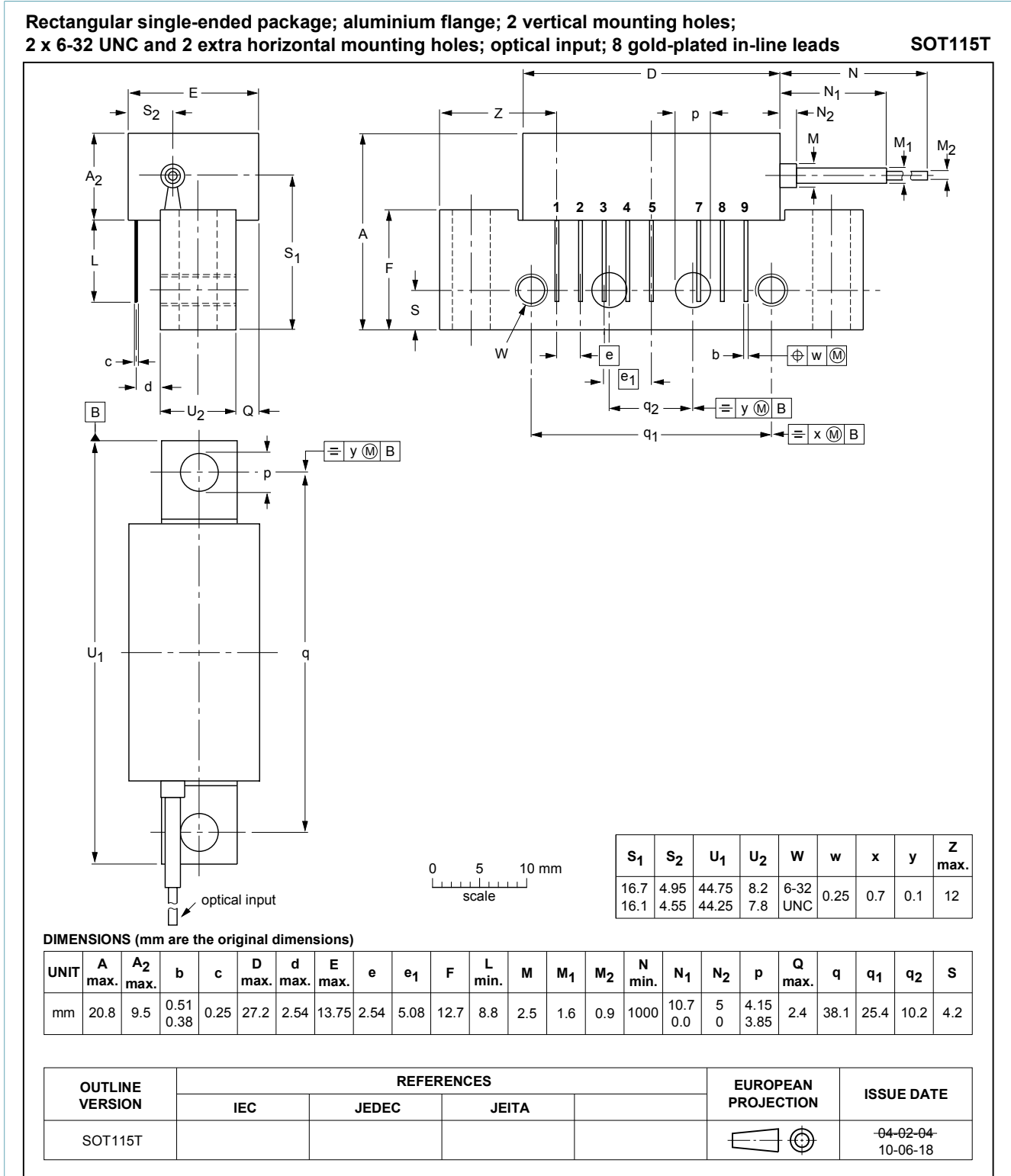
Fig. 1. Package outline SFO8 (SOT115T)
