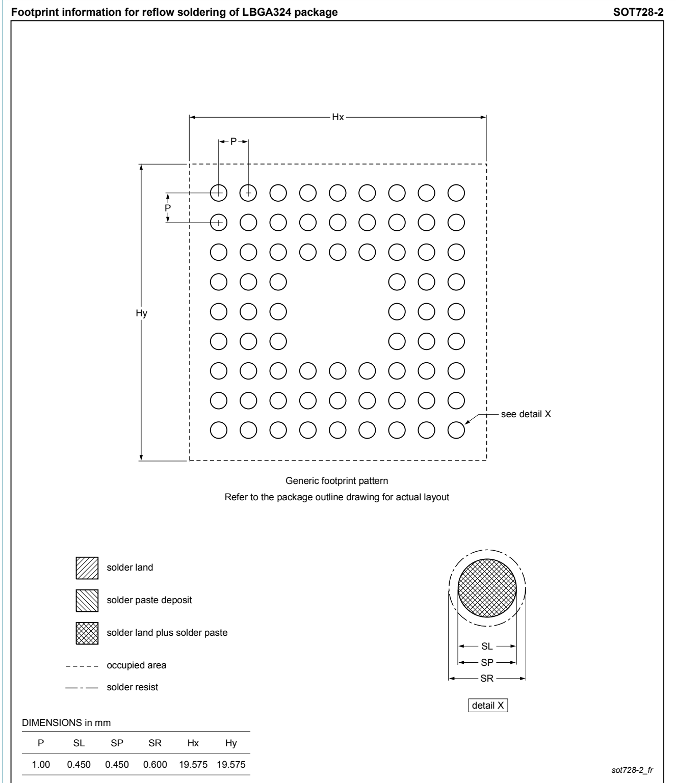
Figure 2. Reflow soldering footprint for LBG324 (SOT728-2)
