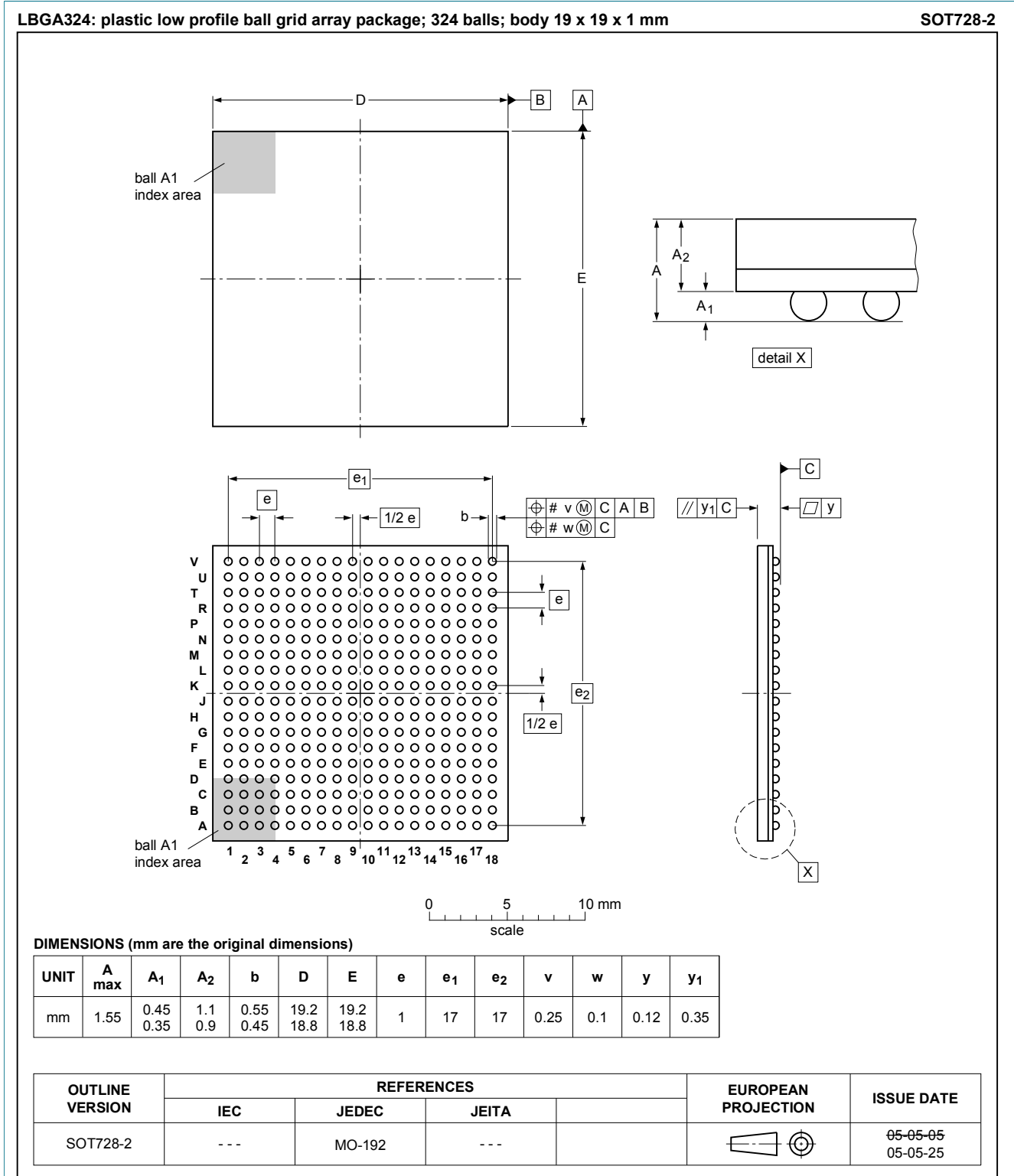
Figure 1. Package outline LPGA324 (SOT728-2)
