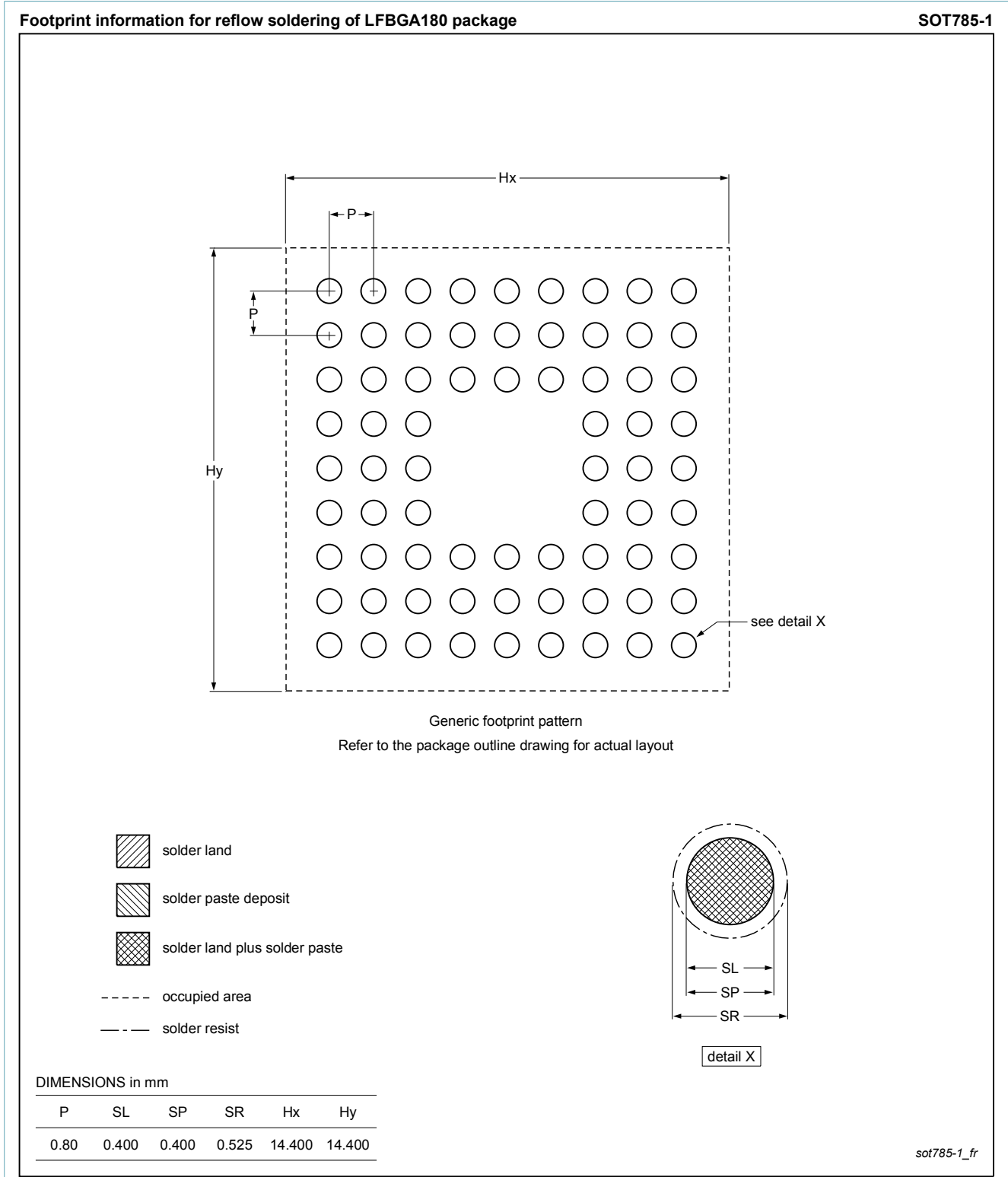
Fig. 2. Reflow soldering footprint for LFBGA180 (SOT785-1)
