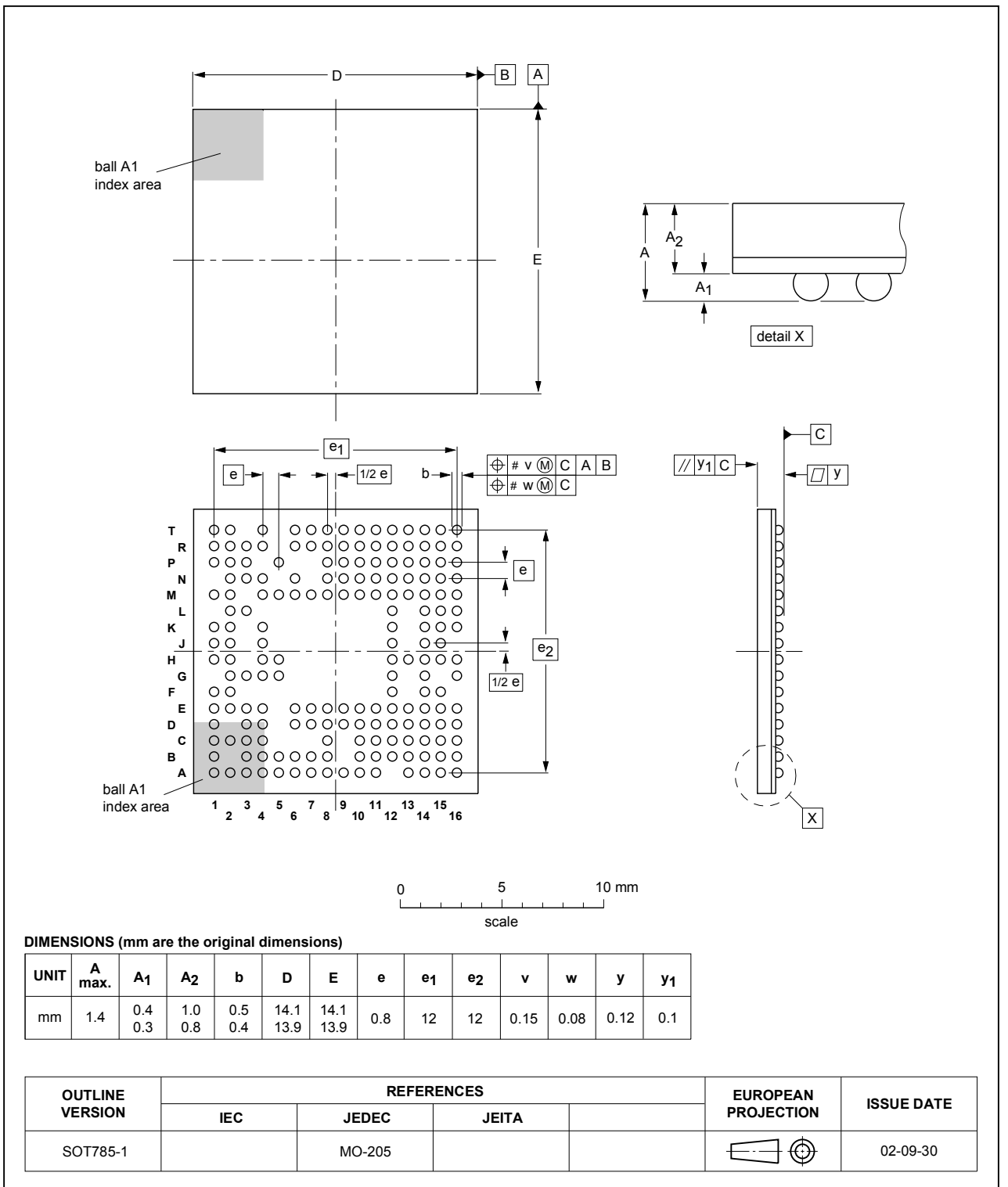
Fig. 1. Package outline LFBGA180 (SOT785-1)
