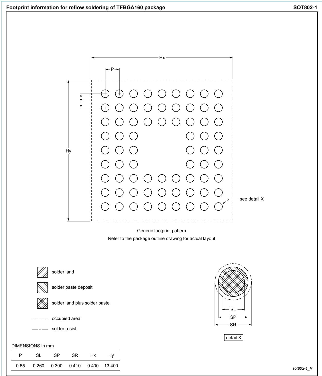
Fig. 2. Reflow soldering footprint for TFBGA160 (SOT802-1)
