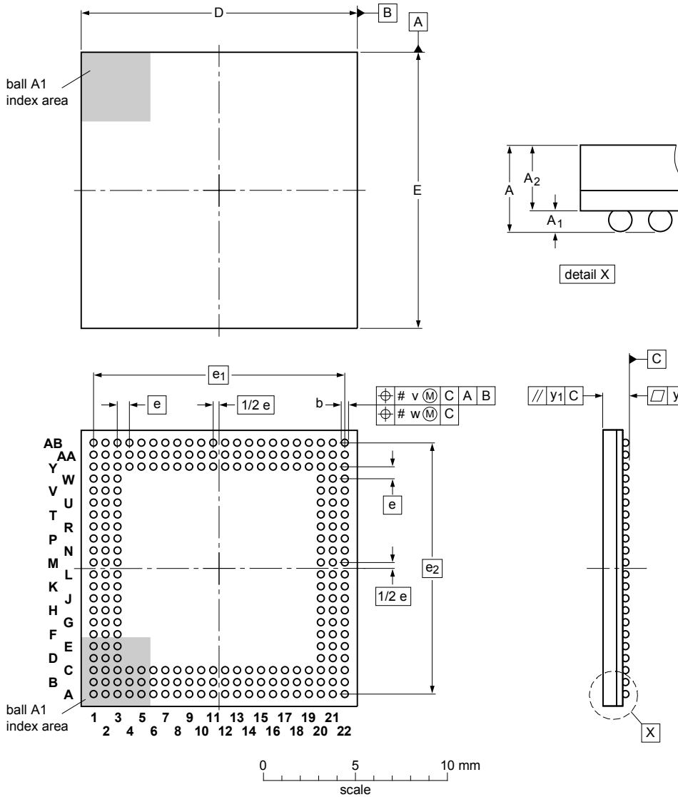
DIMENSIONS (mm are the original dimensions)
