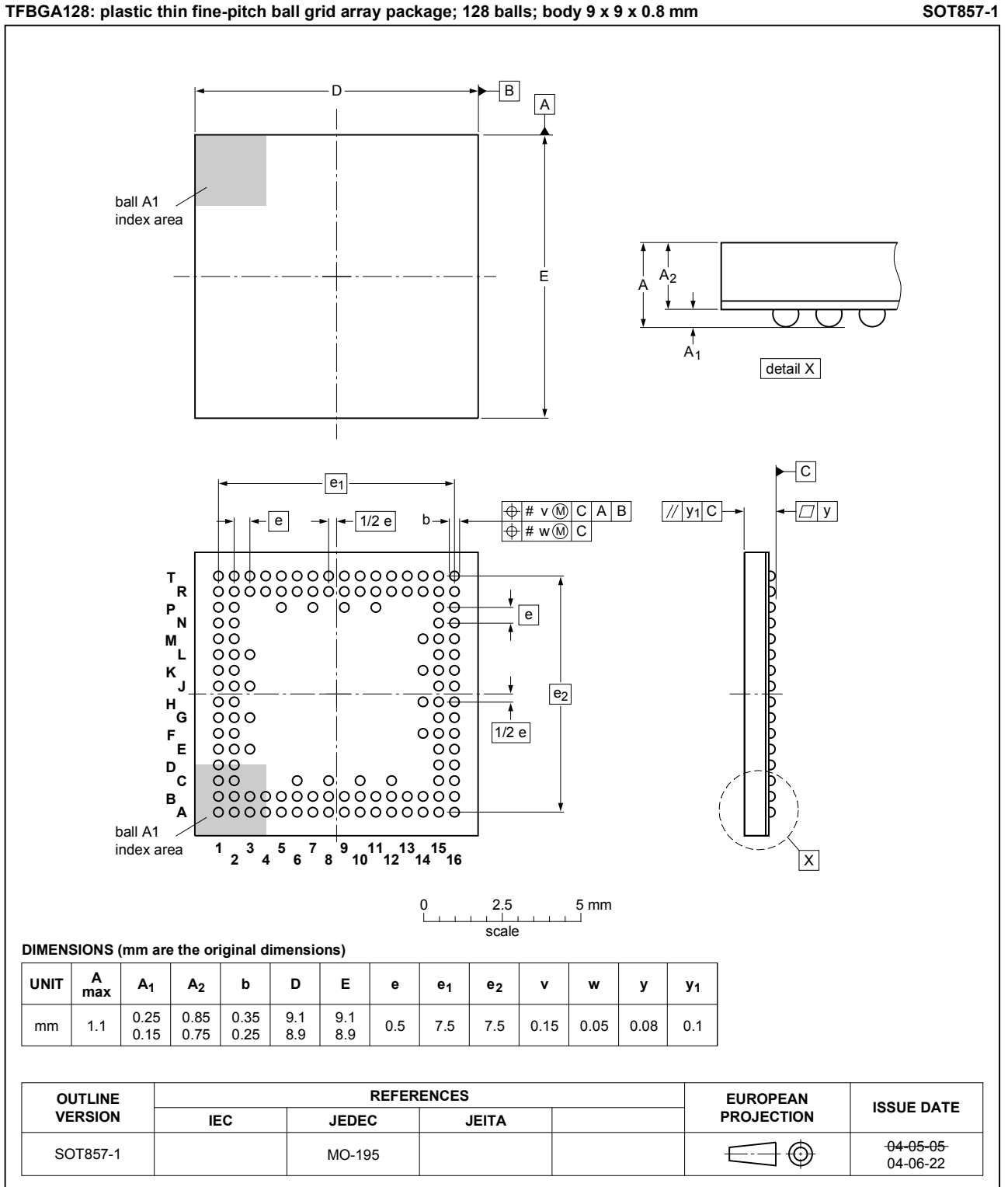
Fig. 1. Package outline TFBGA128 (SOT857-1)
