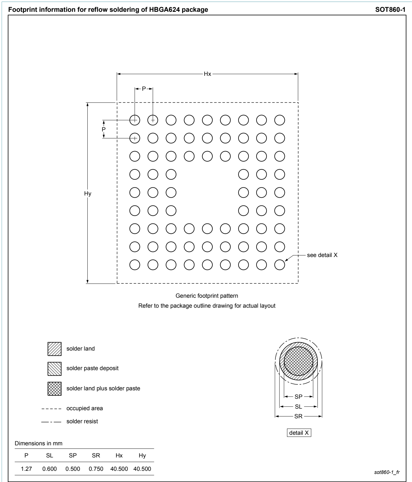
Fig. 2. Reflow soldering footprint for HBGA624 (SOT860-1)
