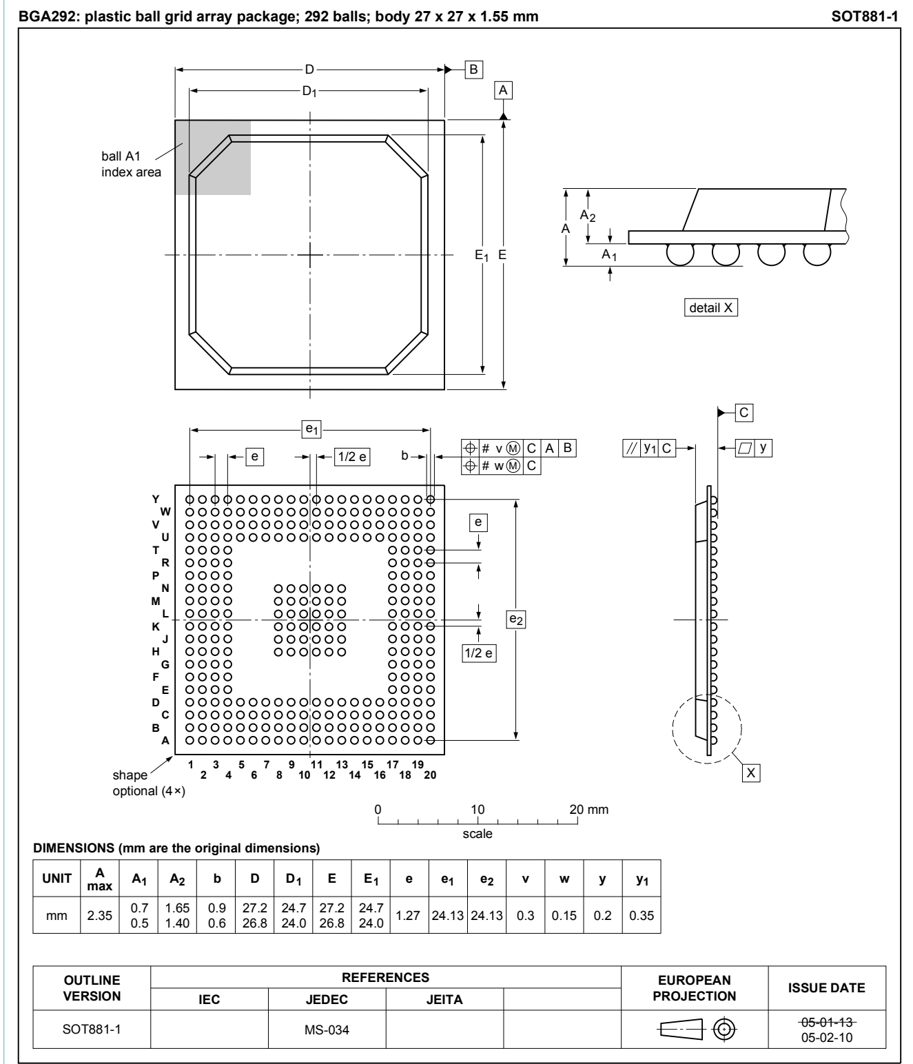
Fig. 1. Package outline BGA292 (SOT881-1)
