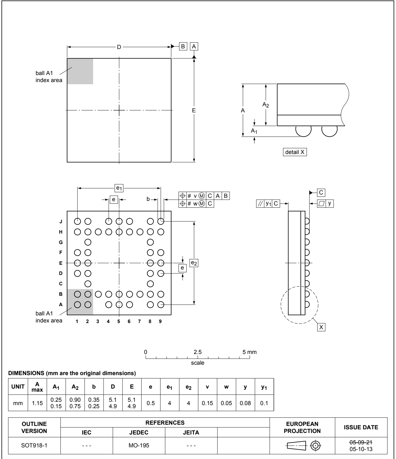
Fig. 1. Package outline TFBGA48 (SOT918-1)
