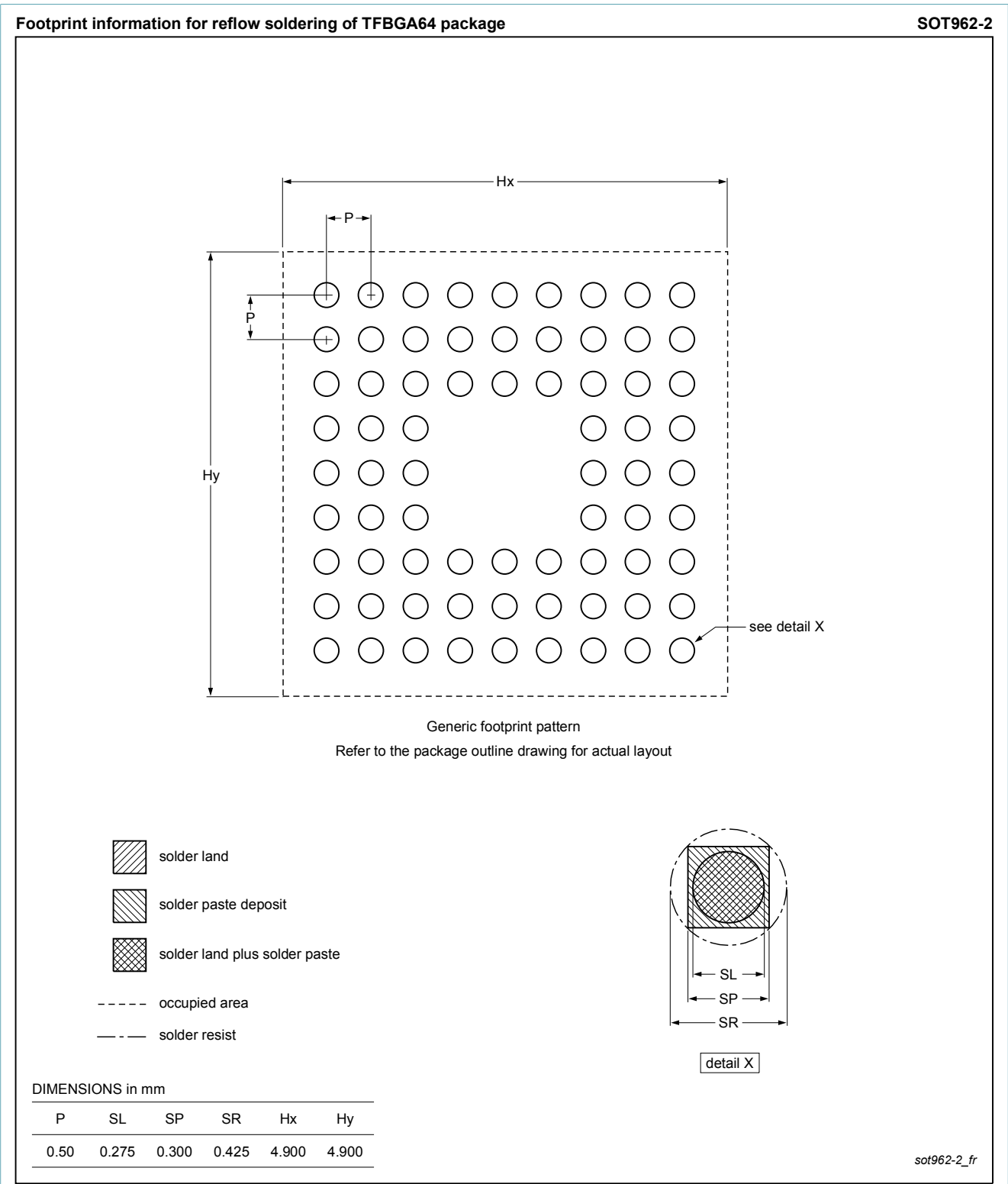
Fig. 2. Reflow soldering footprint for TFBGA64 (SOT962-2)
