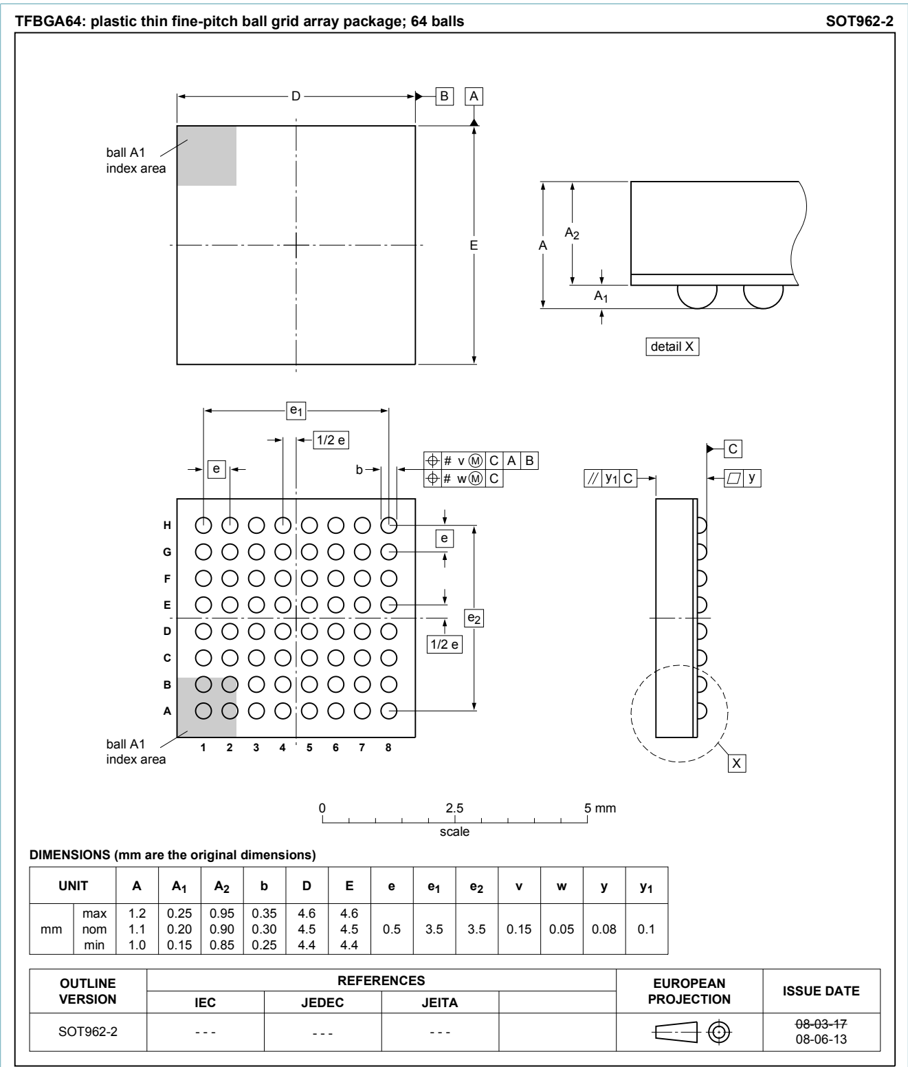
Fig. 1. Package outline TFBGA64 (SOT962-2)
