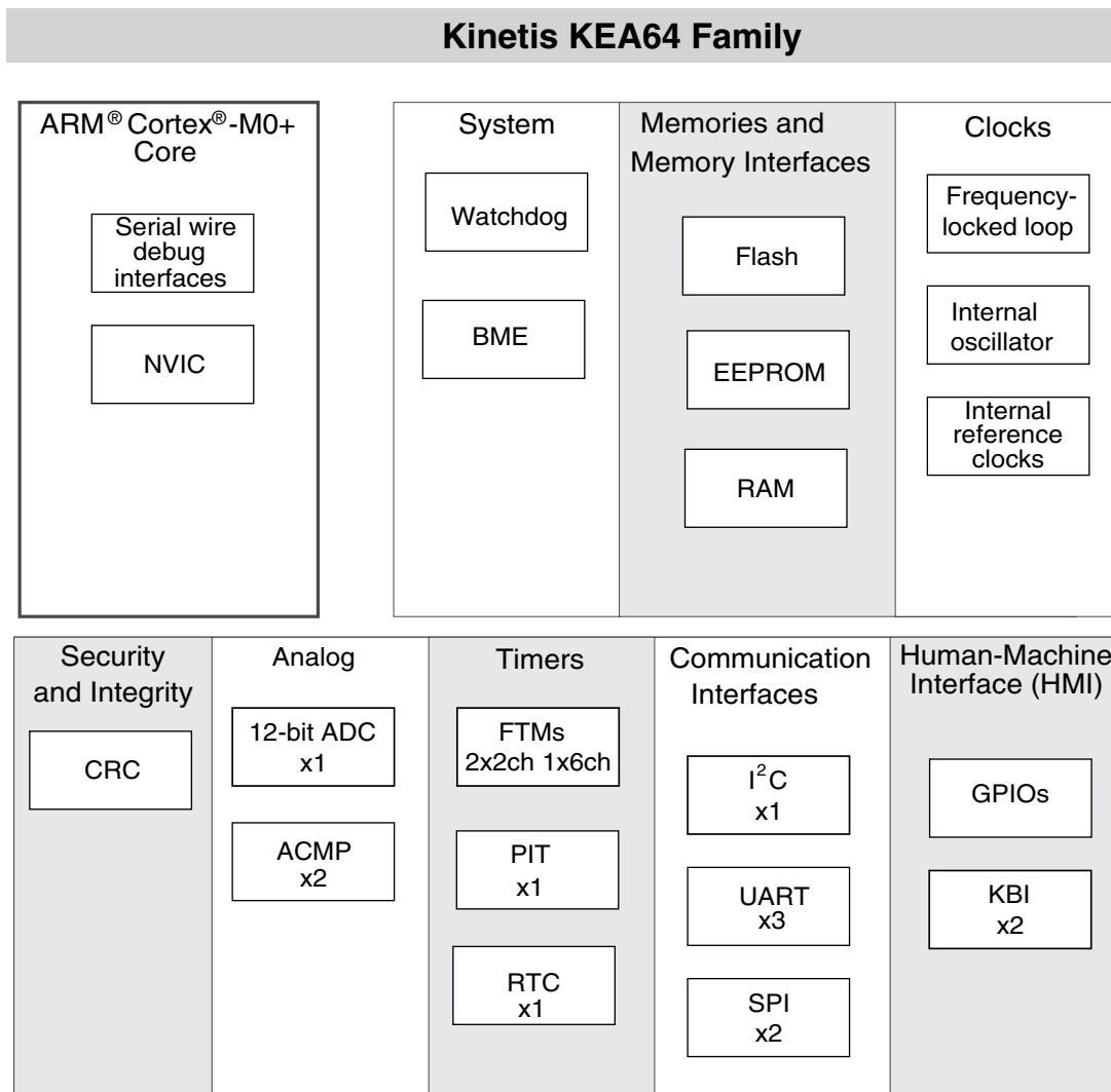
Figure 1. KEA64 family block diagram
