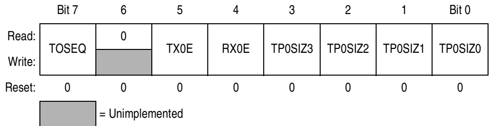
Figure 4-4. USB Control Register 0 (UCR0)
