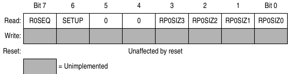
Figure 4-6. USB Status Register 0 (USR0)
