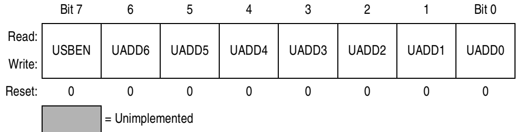
Figure 4-8. USB Address Register (UADDR)
