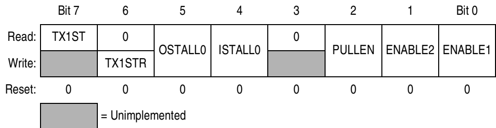
Figure 4-2. USB Control Register 3 (UCR3)
