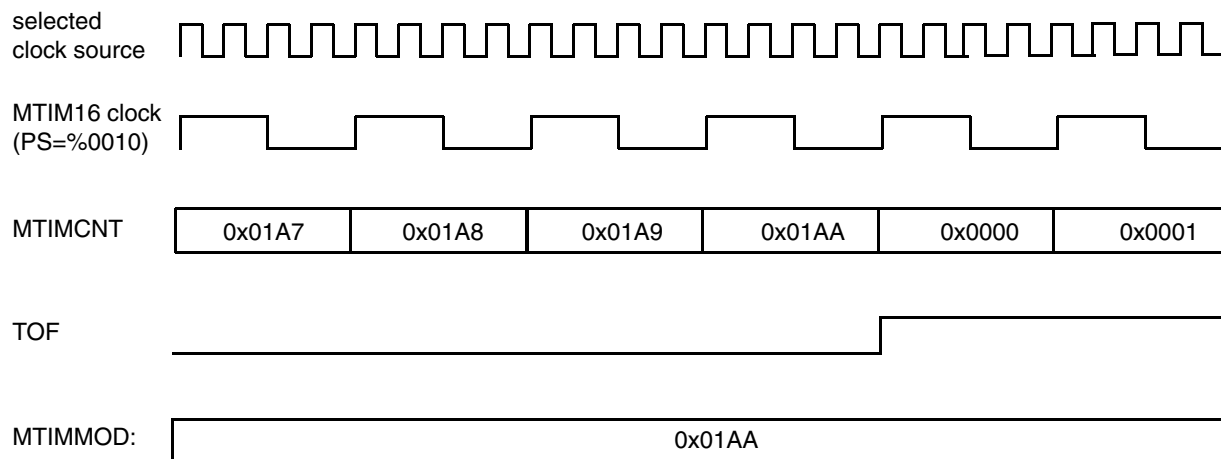
Figure 11-10. MTIM16 Counter Overflow Example
