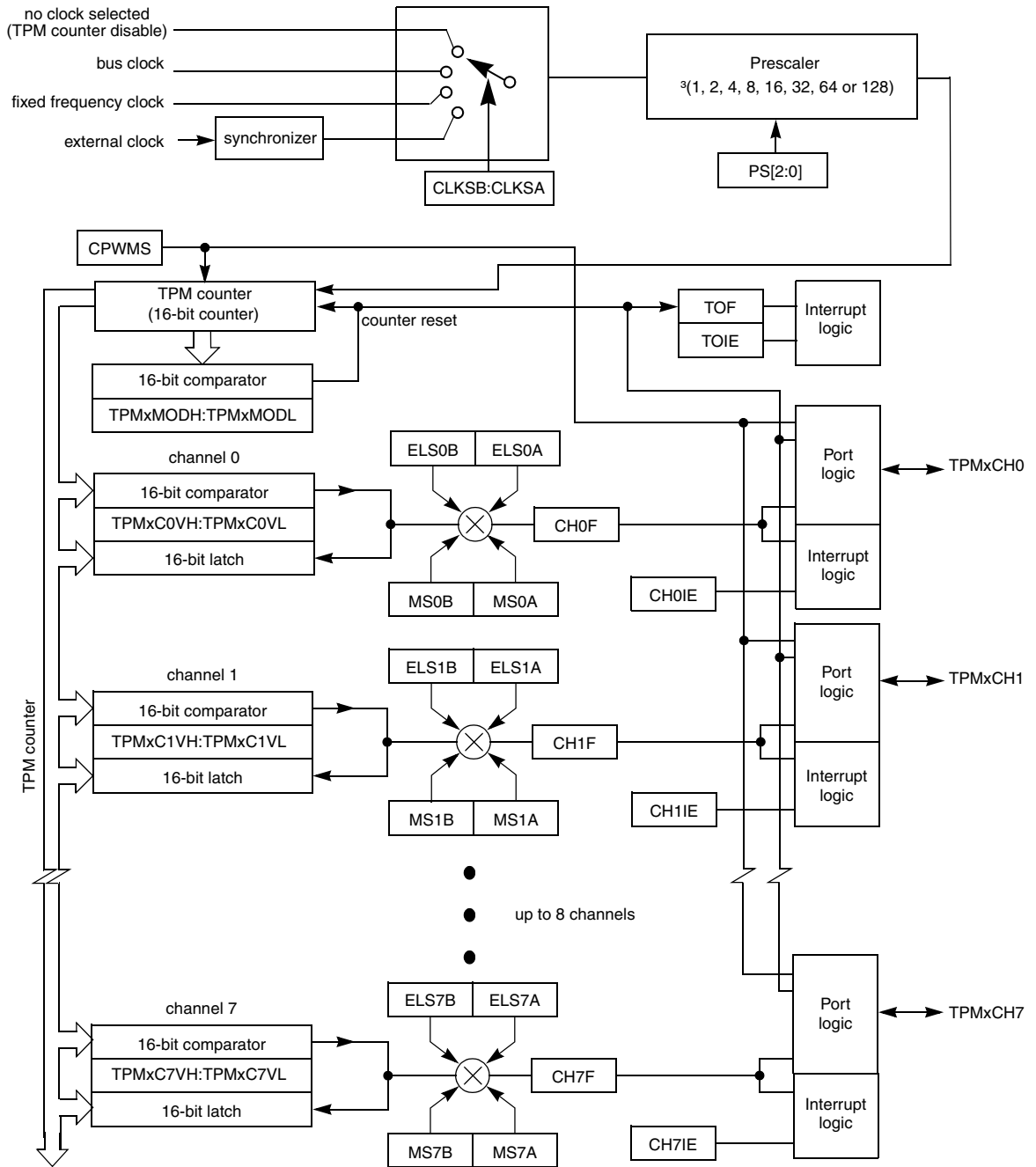
Figure 9-2. TPM Block Diagram
