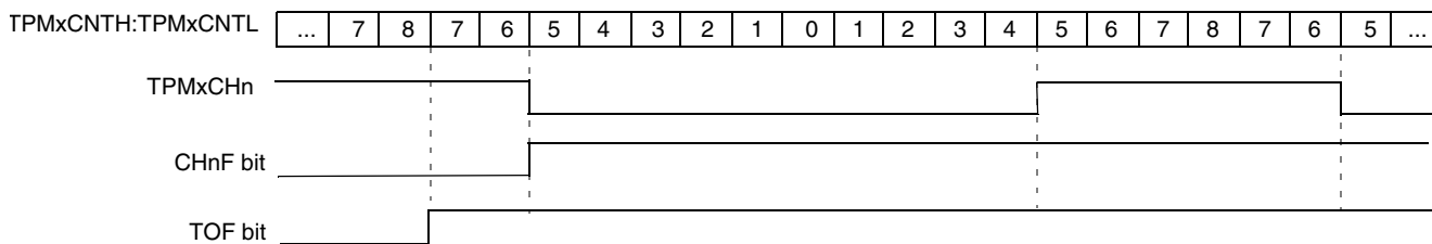
Figure 9-6. Low-true pulse of a center-aligned PWM
