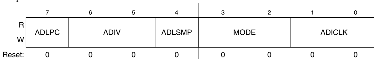
Figure 12-9. Configuration Register (ADCCFG)
