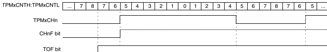
Figure 9-5. High-true pulse of a center-aligned PWM
