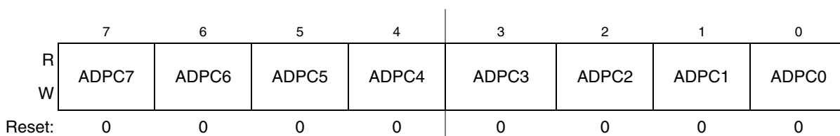
Figure 12-10. Pin Control 1 Register (APCTL1)
