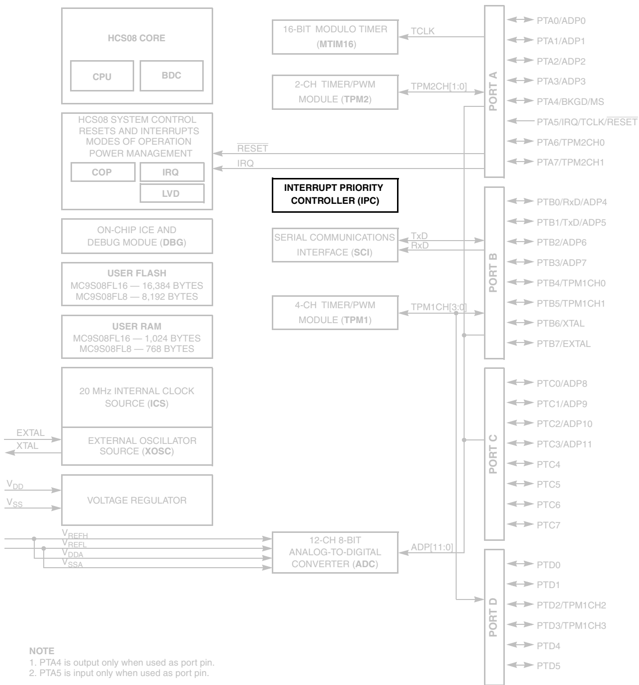
Figure 10-1. MC9S08FL16 Series Block Diagram Highlighting IPC Module
