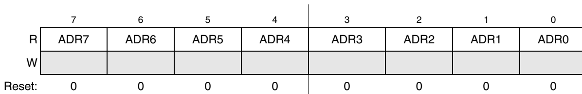
Figure 12-6. Data Result Low Register (ADCRL)
