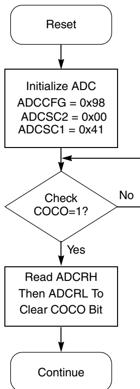
Figure 12-13. Initialization Flowchart for Example
