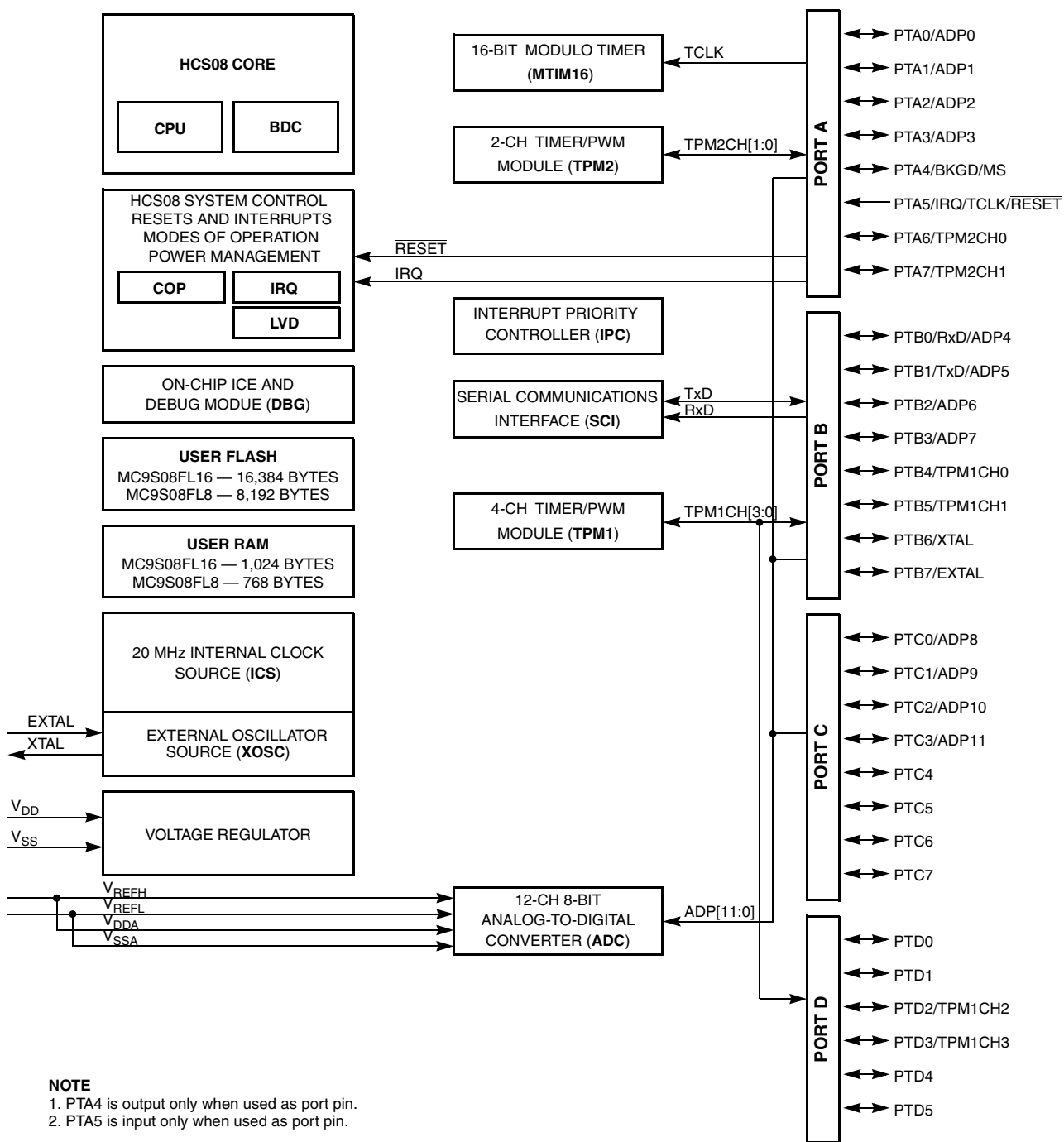
Figure 1-1. MC9S08FL16 Block Diagram
