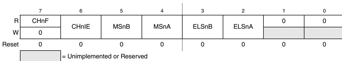
Figure 9-12. TPM Channel n Status and Control Register (TPMxCnSC)
