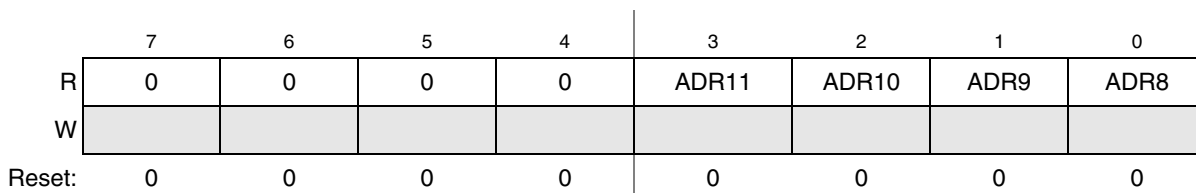
Figure 12-5. Data Result High Register (ADCRH)
