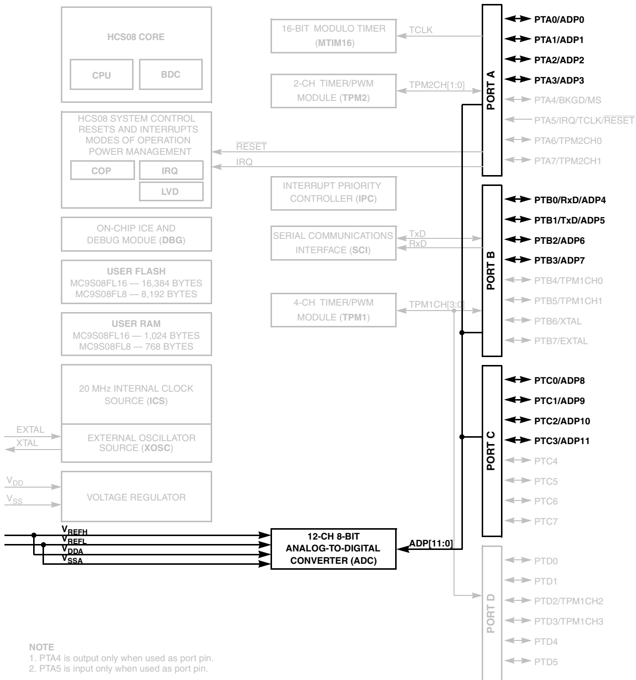
Figure 12-1. MC9S08FL16 Series Block Diagram Highlighting ADC Module and Pins.
