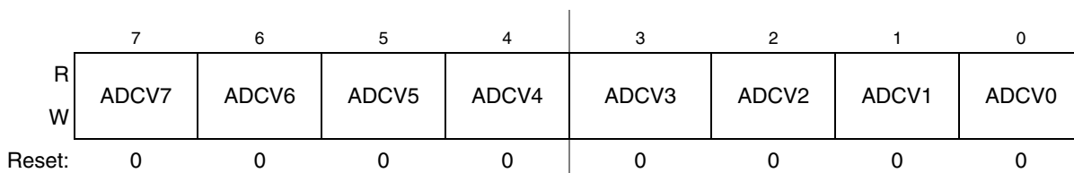
Figure 12-8. Compare Value Low Register (ADCCVL)
