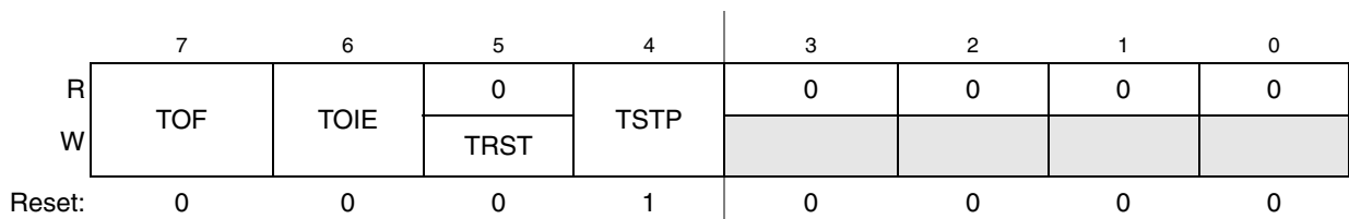
Figure 11-4. MTIM16 Status and Control Register (MTIMSC)
