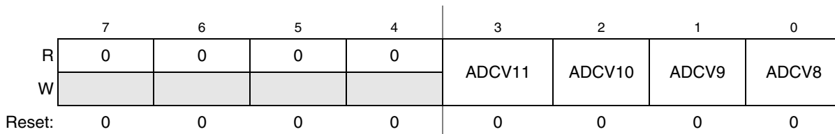
Figure 12-7. Compare Value High Register (ADCCVH)
