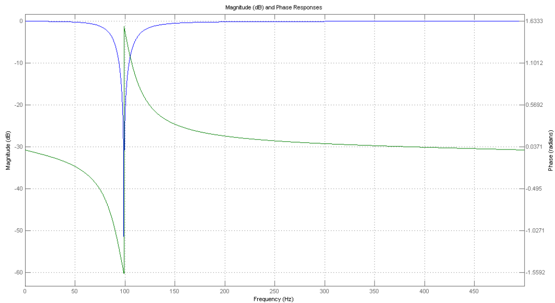
Figure 32. Filter response
