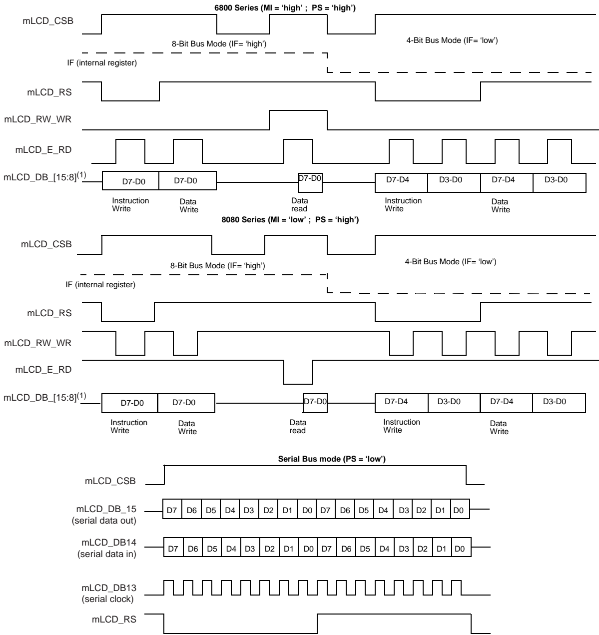
Fig 68. Timing diagram
