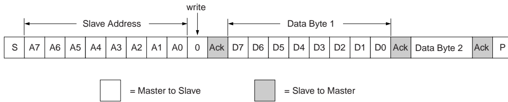
Fig 77. I 2 C 7-bit slave address write operation
