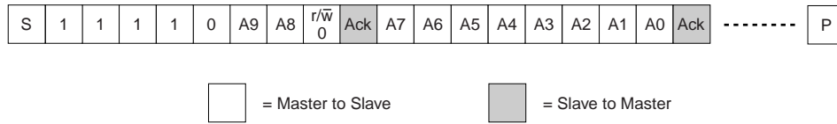
Fig 76. I 2 C 10-bit device addressing
