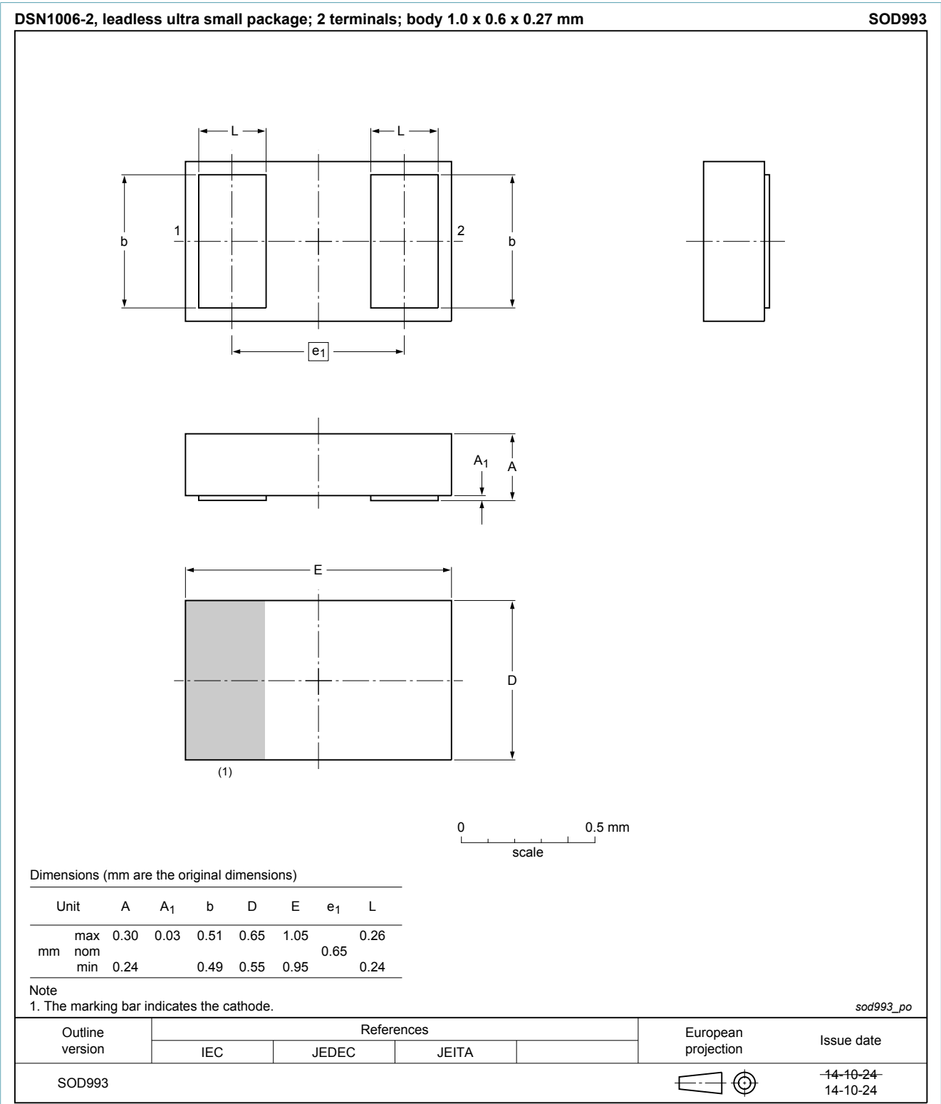
Fig. 1. Package outline DSN1006-2 (SOD993)
