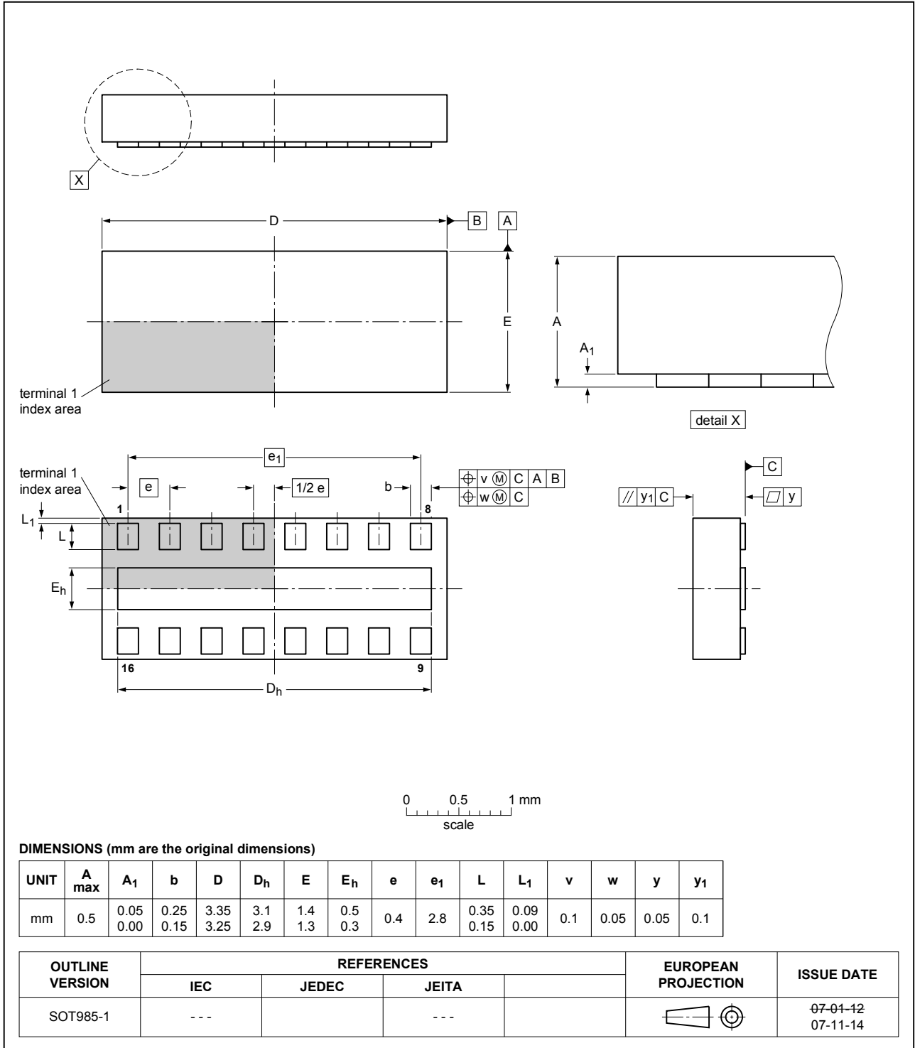
Fig. 1. Package outline DFN3314U-16 (SOT985-1)
